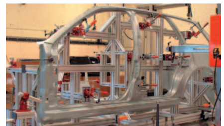
Clamping and measuring device
